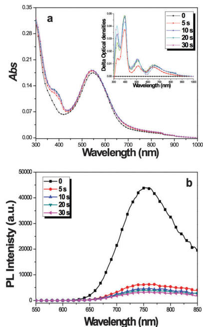
Fig. 5 (a), UV-vis and (b), fluorescence spectra of PMI-N-HABI in the film under irradiation of 302 nm with the time varying from 0, 5, 10, 20 to 30 s; the inset in (a) is the changes of optical absorption with different irradiation time.
